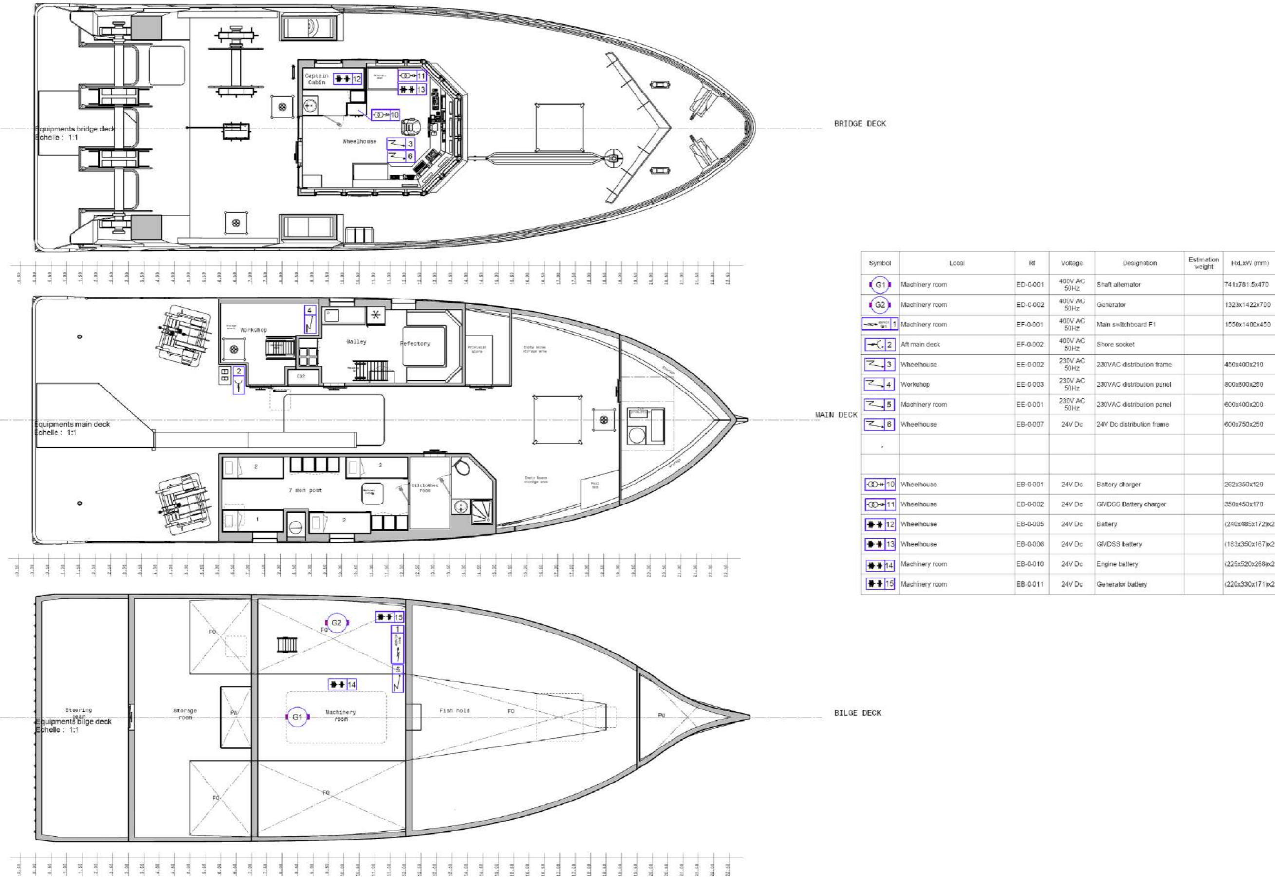
Figure 7-20 Electric Equipment Location
