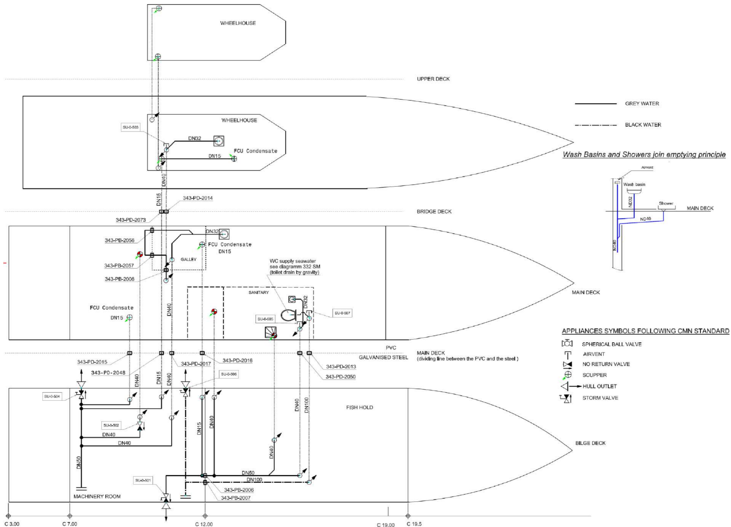
Figure 7-11 Sewage System
