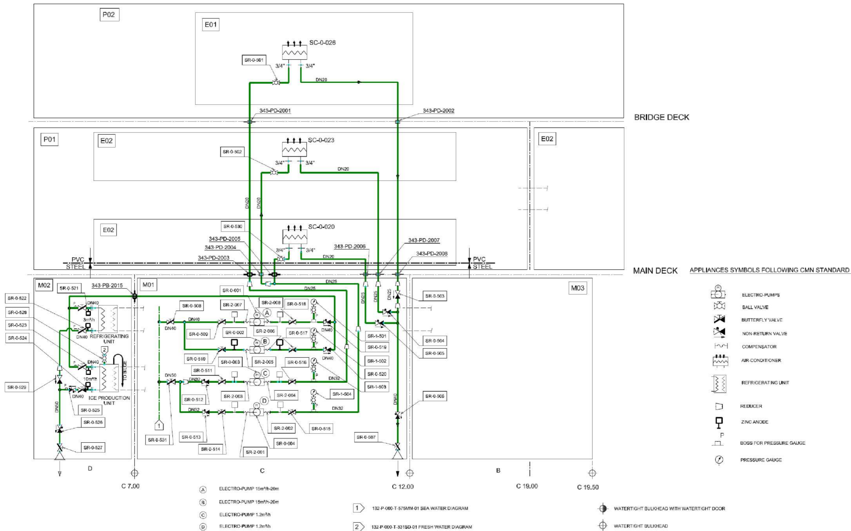
Figure 7-5 AC Sea Water Cooling System
