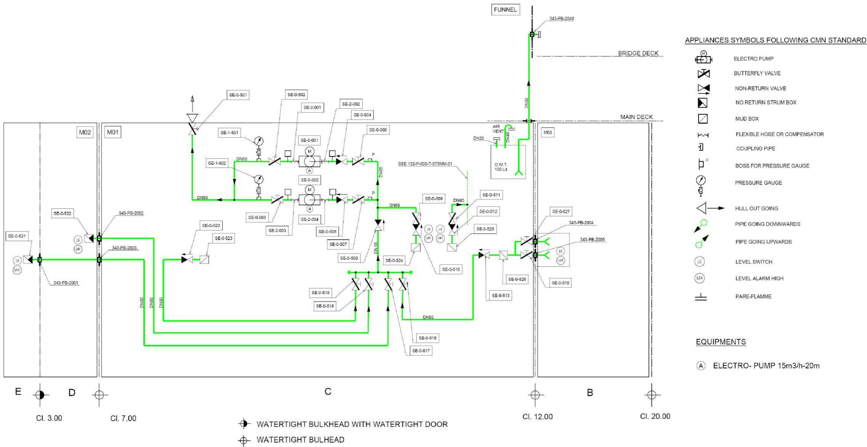
Figure 7-10 Bilge System
