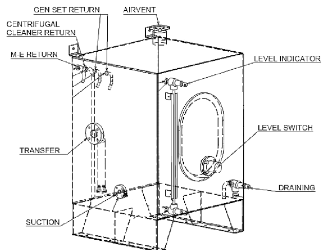
Figure 5-20 Engine Room - Fuel Oil Service Tank
