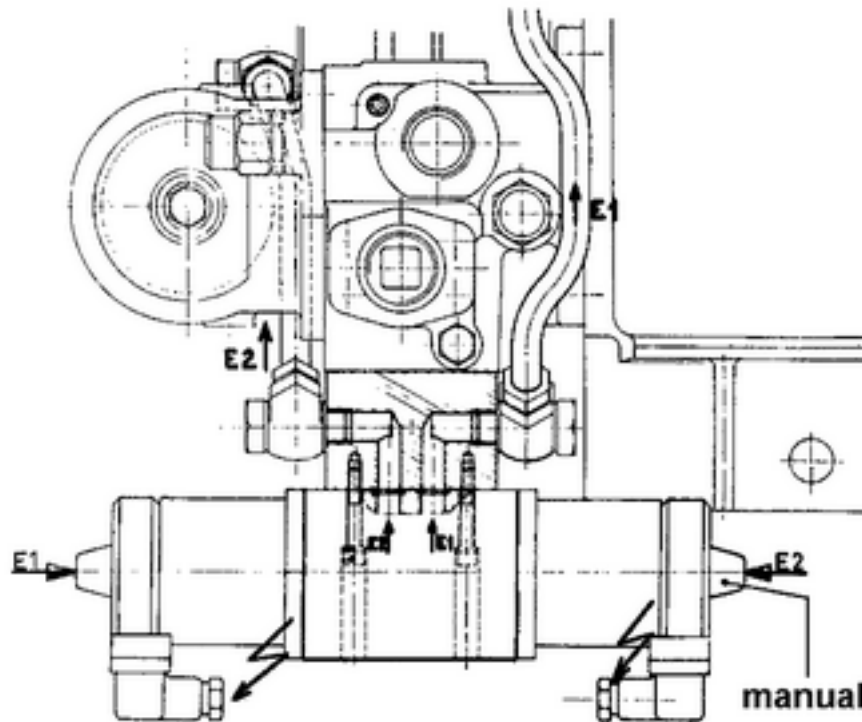
Figure 5-41 Engine Room - Manual Clutching of Propeller Shaft
