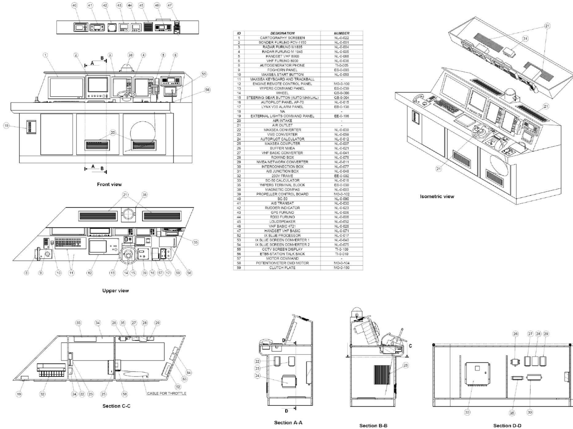
Figure 7-32 Wheelhouse Fwd Console
