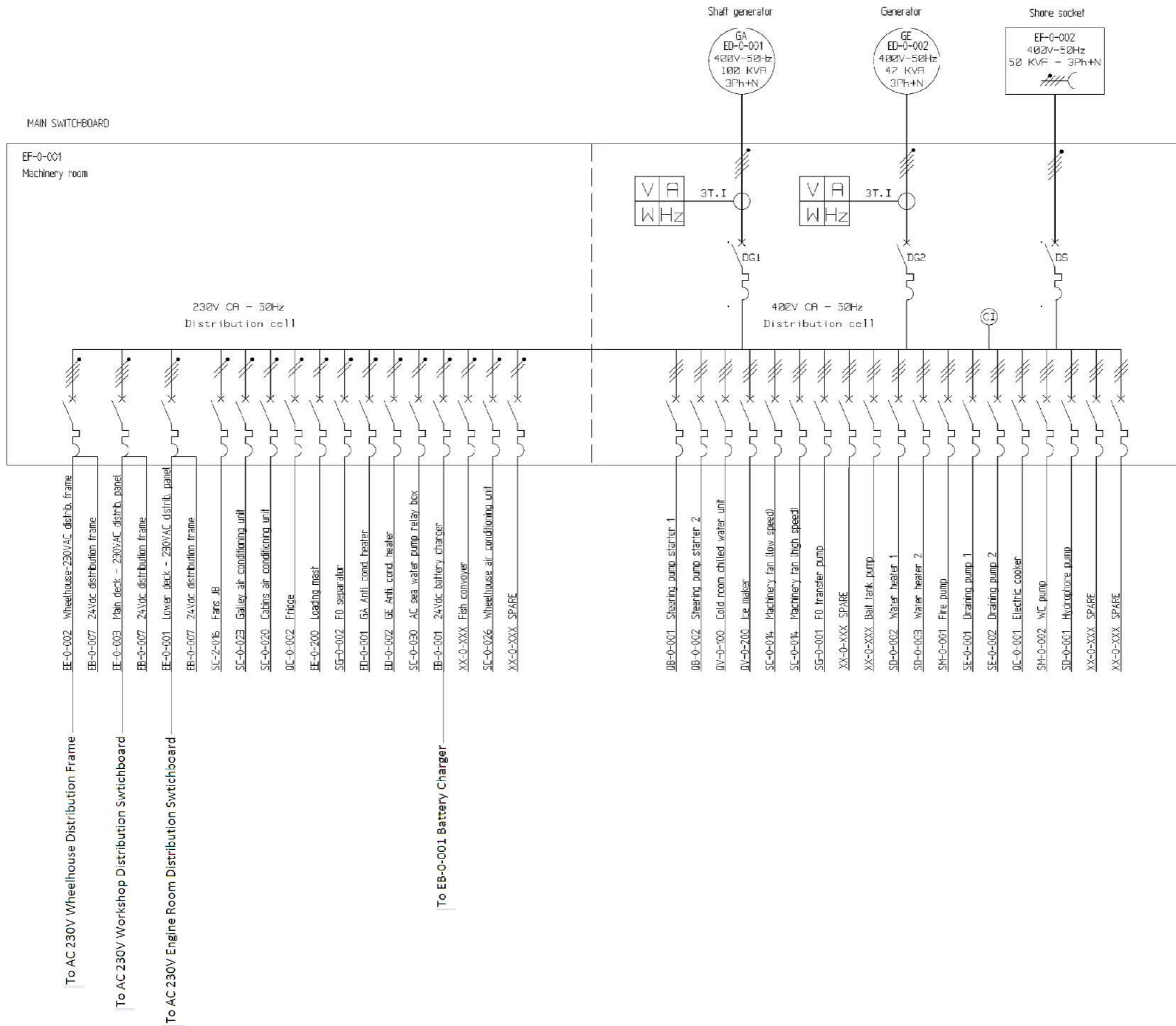
Figure 7-22 Main Switchboard Diagram
