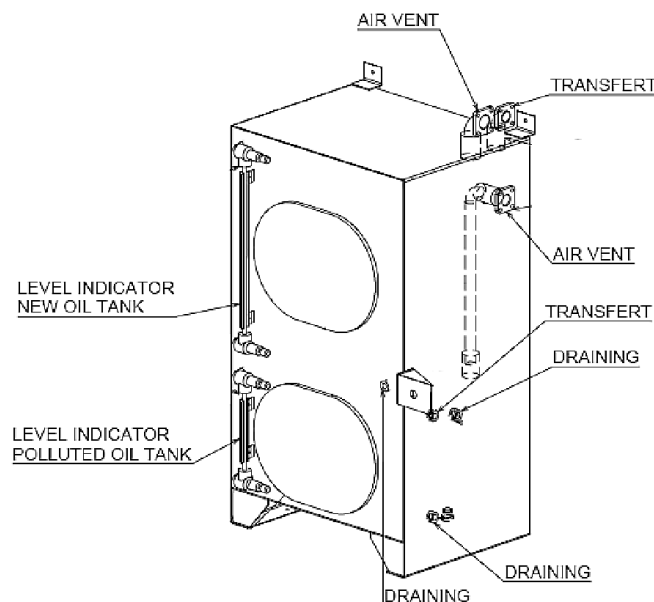
Figure 5-22 Engine Room - New Oil & Polluted Oil Tanks
