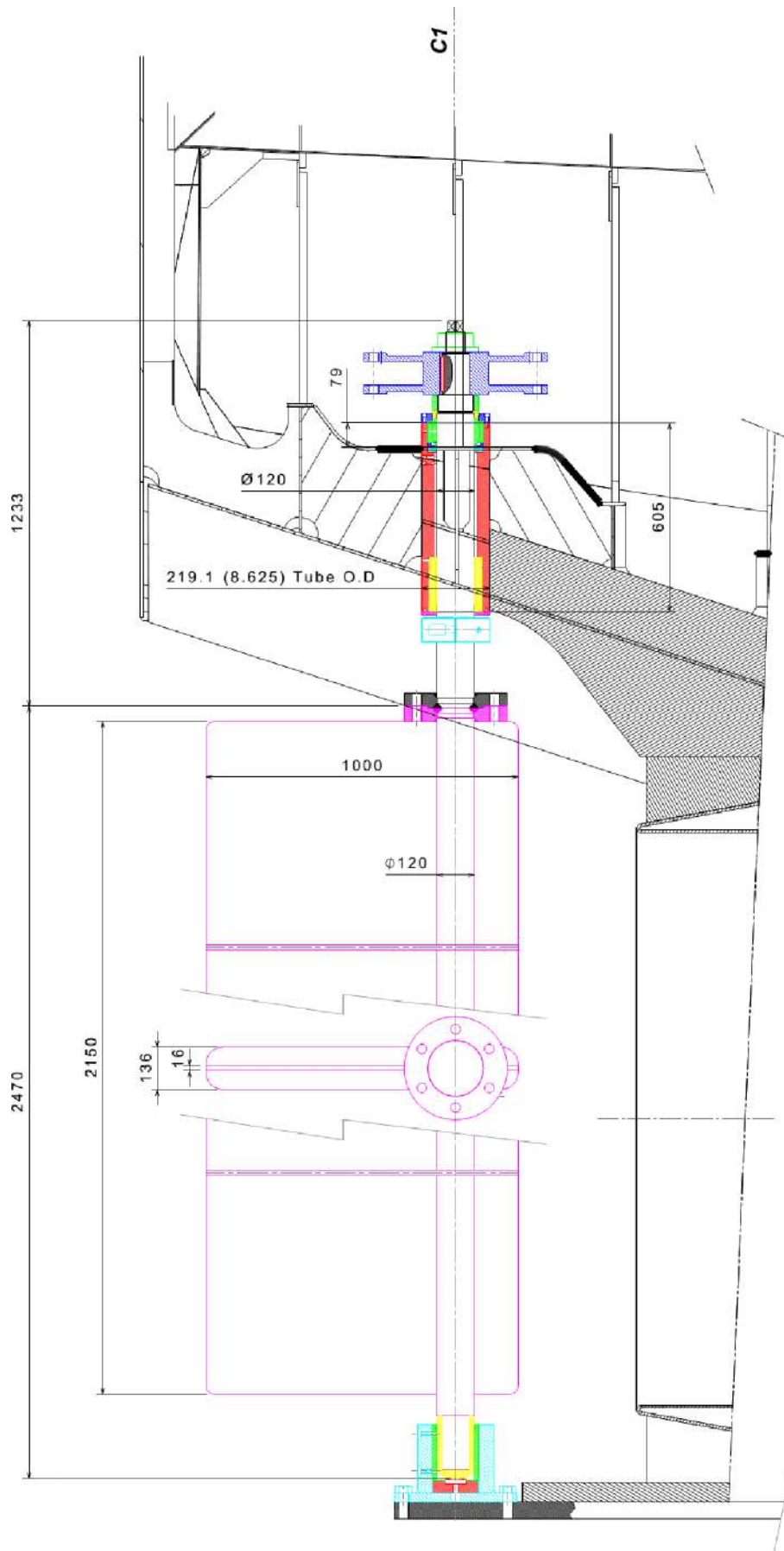
Figure 7-2 Rudder Stock
