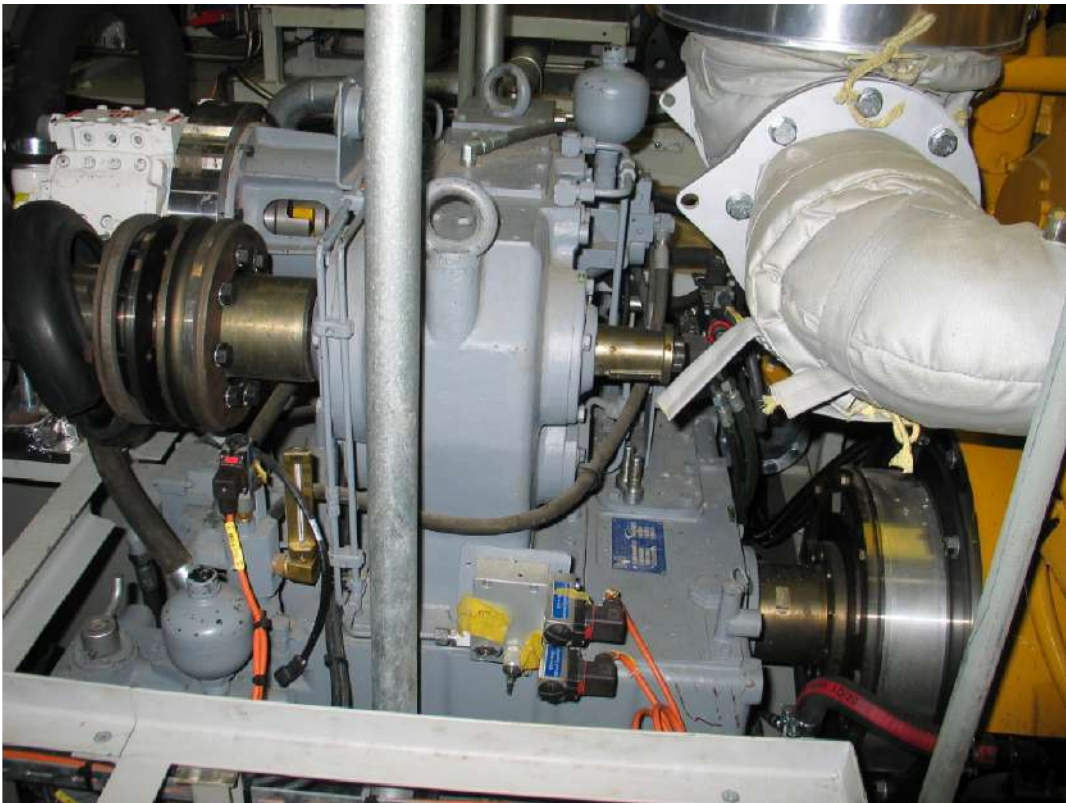
Figure 2-47 Engine Room - Reduction Gearbox
